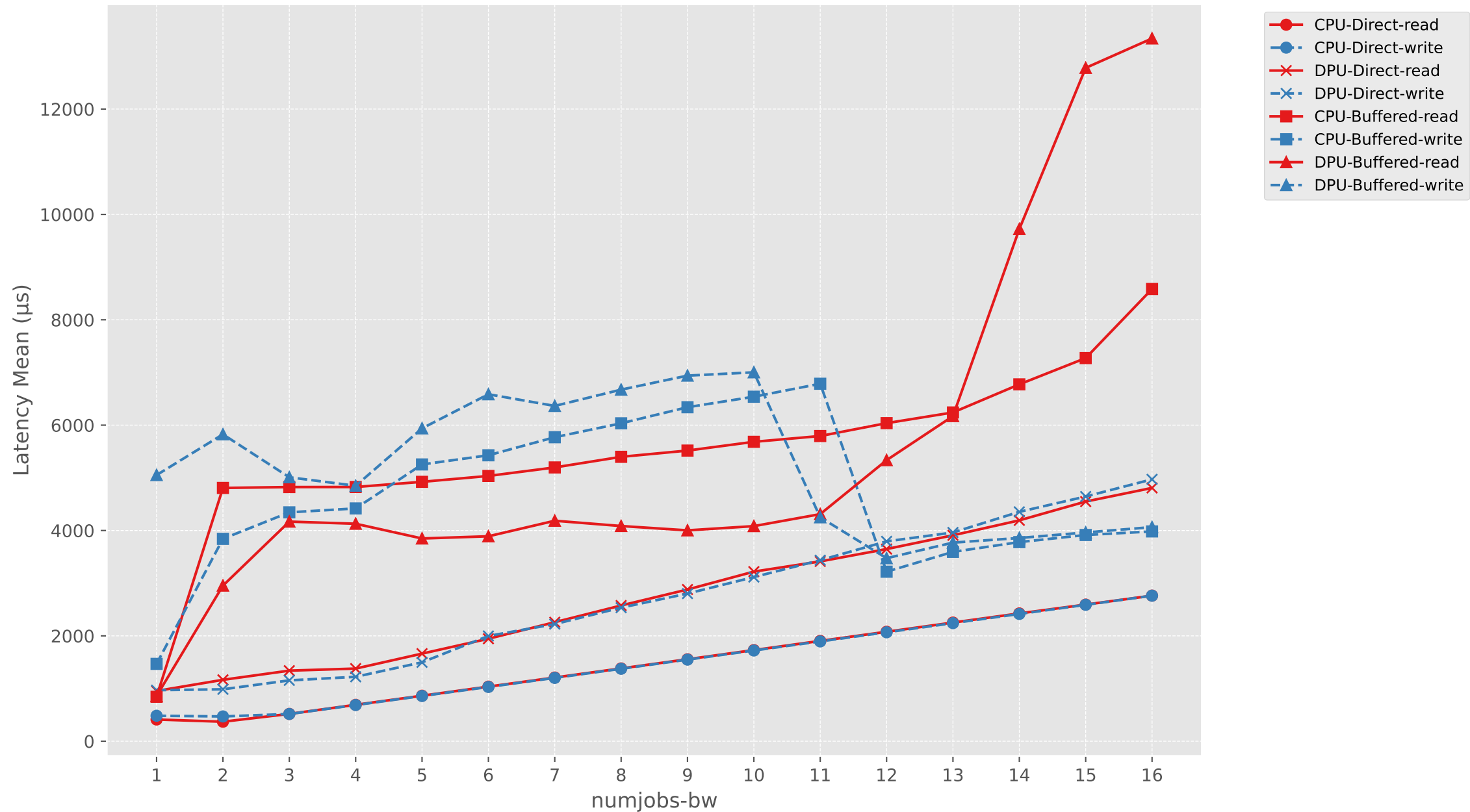
Latency Mean vs numjobs-bw (CPU vs DPU, Direct vs Buffered)
